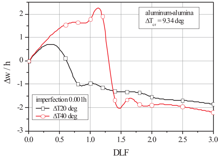
Figure 8 Dynamic response of FGM plate subjected to thermo–mechanical loads
