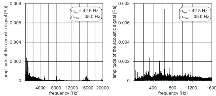
Figure 6 Main components of the acoustic signal of both rotors in function of frequency for fan rotational speed n_f = 42.5 Hz and rotor rotational speed n_r = 35.0 Hz; left side: whole acoustic range of the signal; right side: more detailed image of the lower part (up to 1600 Hz) of the acoustical frequency range
