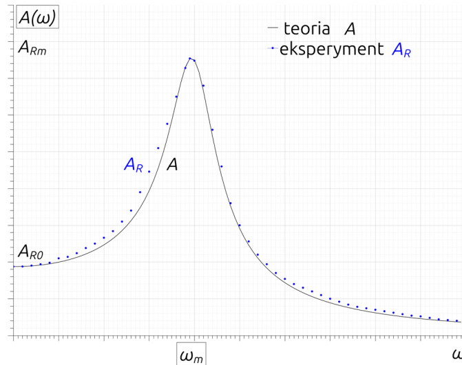
Figure 3: Resonance curves
