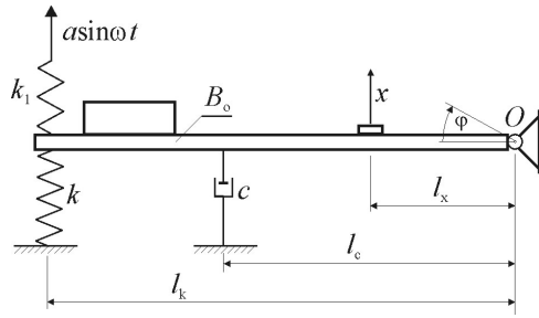
Figure 1: Schematic diagram of the vibrating system
