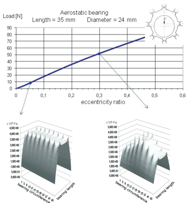
Figure 1 Design of the aerostatic bearing and the calculated load characteristics and a gas film pressure distribution of the externally pressurized gas bearing
