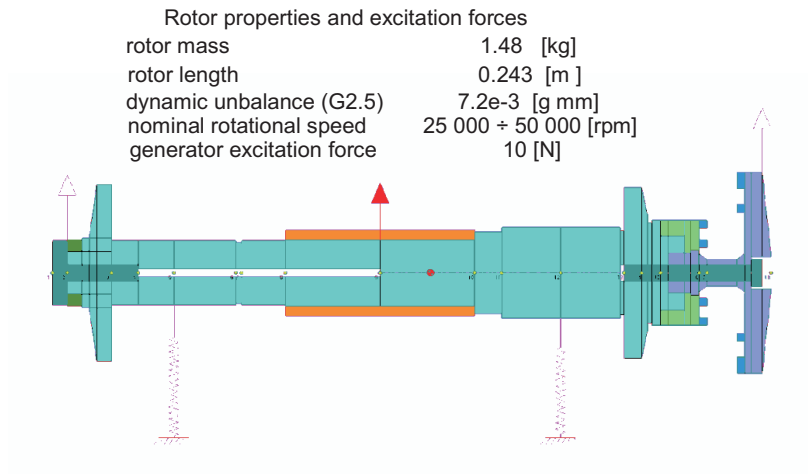
Figure 4 Numerical model used for rotor–dynamic calculations of the turbogenerator developed for the ORC cycle
