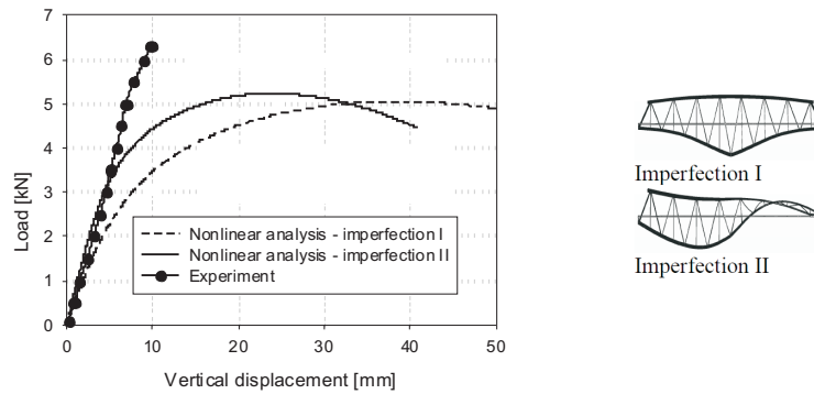
Figure 12 The truss loading at one top chord joint vs. the vertical displacement (at 0,75 m from the mid-span) of truss with 3 braces k = 10 \text{ kN/m}
