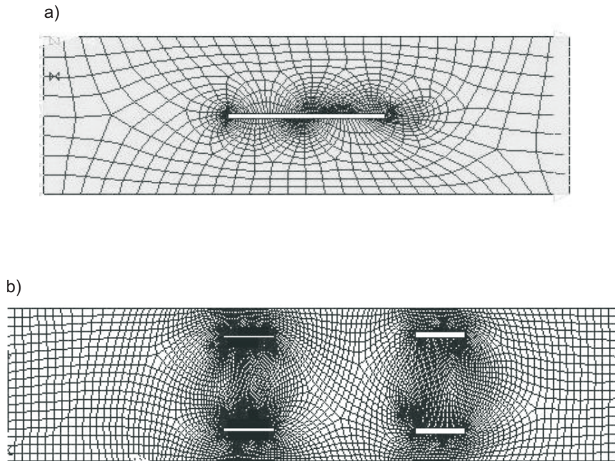
Figure 3 a) Model with one central fissure, b) Model with four fissures
