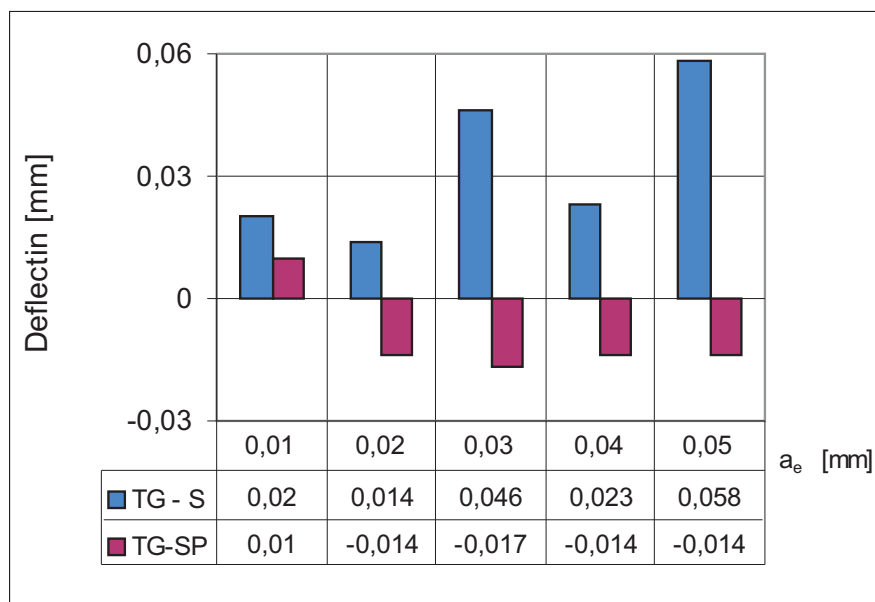
Figure 6 Comparison of deflections for the titanium alloy Ti6 Al4V, grinding wheel 5TGP with SP-compressed air, S – without cooling
