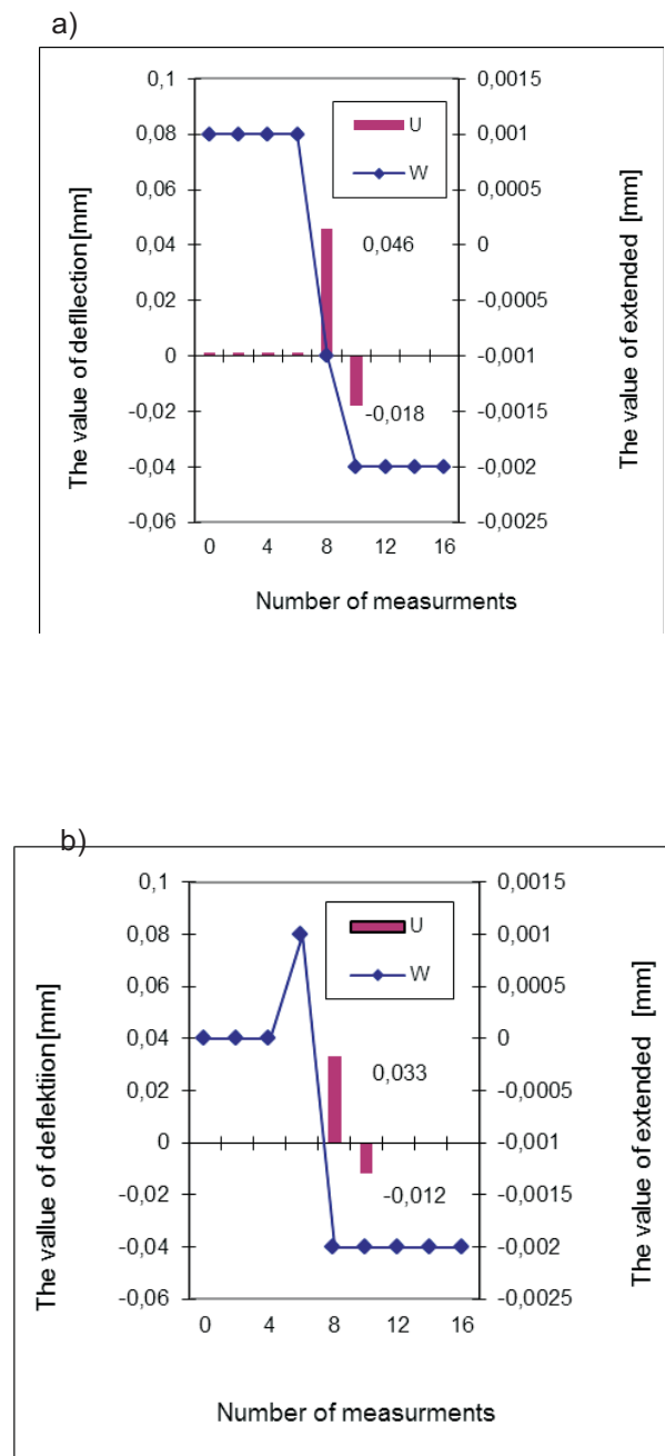
Figure 5 Comparison of deflection and elongation for alloy Ti6 Al4V with grinding wheel 5TGP using oil mist, a_e = 0,03 \text{ mm} : a) v_w = 0,1 \text{ m/s} , b) v_w = 0,5 \text{ m/s}
