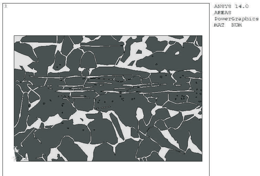
Figure 6 Finite element mesh of the model
