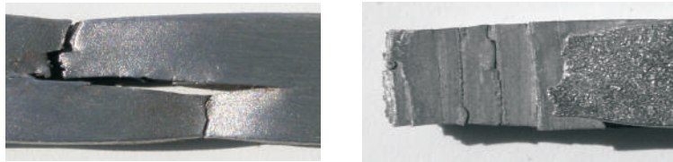
Figure 2 View of the sample just before tearing and after tearing of the samples
