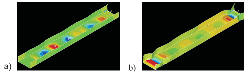
Figure 18 The structural failure form for DLF=2.6 T66 for Perzyna Model (a) and experimental characteristic (b)
