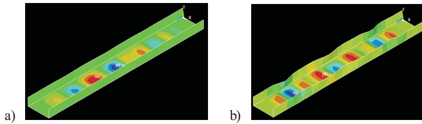
Figure 13 Dynamic buckling mode of the T4 C-profile a) DLF = 1.4 and b) DLF = 2.6
