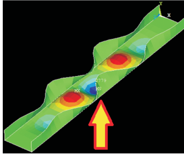
Figure 10 Location of characteristic node, the vertical deflection and critical buckling load achieved by Eigen Buckling Analysis
