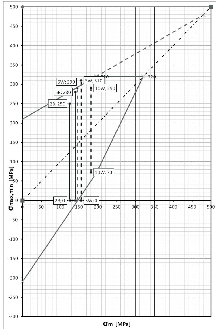
Figure 7 Smith graph with marked fatigue tests, where samples were not damaged
