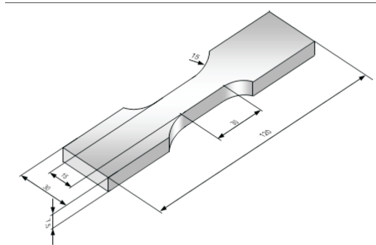
Figure 3 The dimensions of the samples taken for testing
