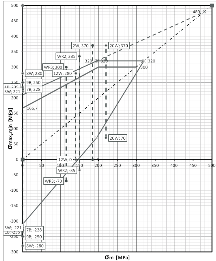
Figure 6 Smith graph with marked fatigue tests in which samples of them were destroyed
