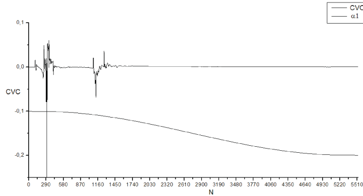
Figure 14 Time series of the links angular displacements and CVC parameter – link 1
