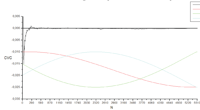
Figure 9 Time series of the links angular displacements and CVC parameter – links 4 and 6
