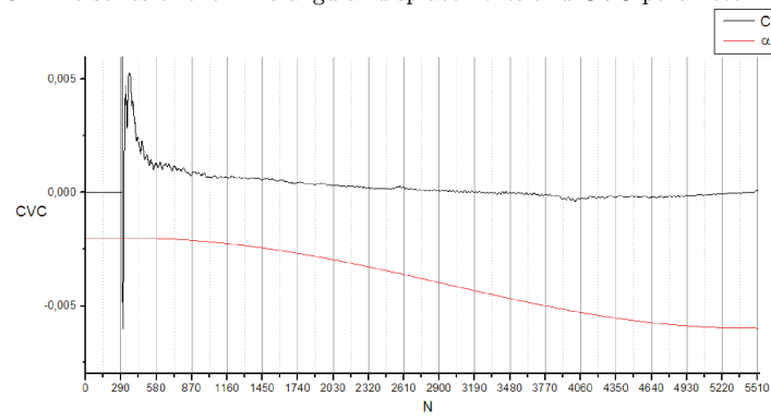
Figure 6 Time series of the links angular displacements and CVC parameter – link 2
