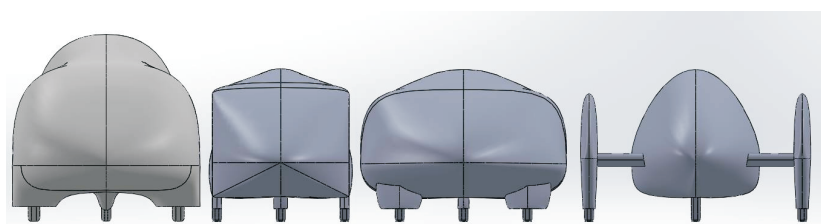
Figure 6 Car body shapes with fairings: a) Eco-Arrow; b) Prototype 1; c) Prototype 2; d) Prototype 3
