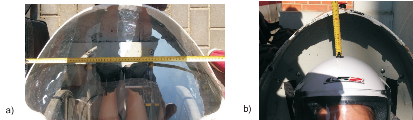
Figure 3 Measurement of the current car body loses: a) width near the feet (on the left); b) height above the helmet (on the right)
