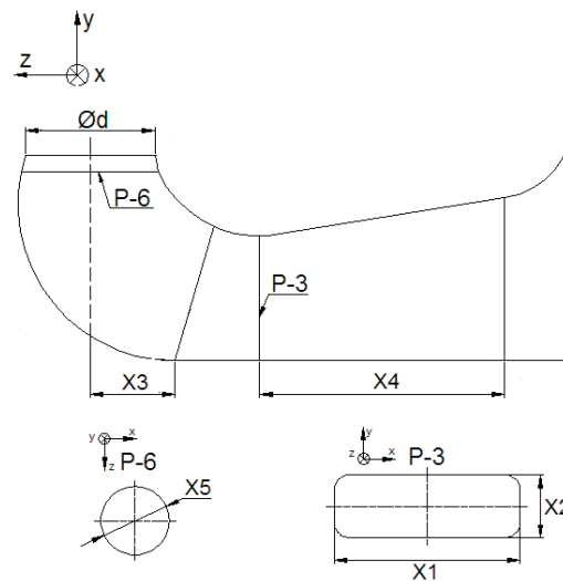
Figure 8 Design variables
