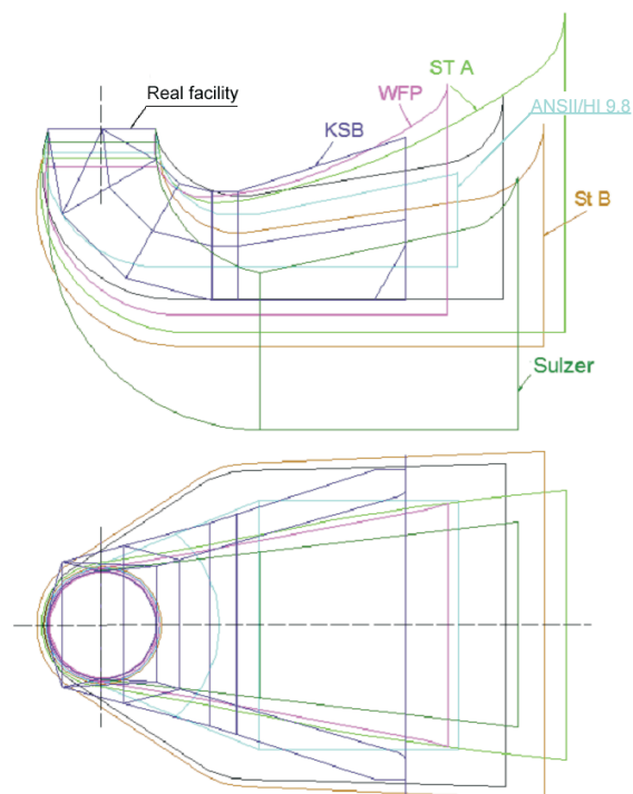
Figure 3 Meridional (a) and longitudinal (b) contours of suction intakes. Comparison to the suction intake in the 458MW unit in Ptnów II Power Plant, Poland [4]
