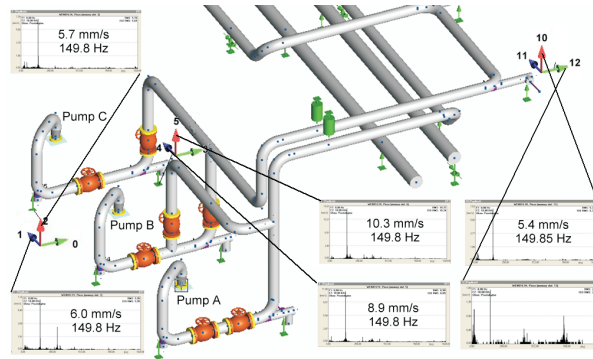
Figure 9 Measuring position of vibrations at discharge pipelines
