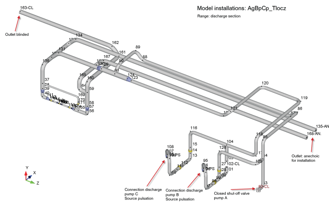
Figure 14 Model #3 labeled A.g.B.p.C.p.272.5: discharge piping system for defined for acoustic analysis in operating case with pumps B & C on and the pump A shut-off valve closed. On piping end 163 is the blind flange, ends 135 and 168 connected to anechoic, long piping system
