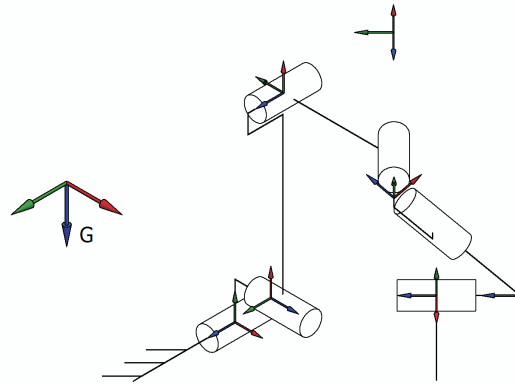
Figure 1 Kinematics of measurement arm
